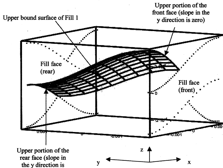
Fig. 5. Illustration of three-dimensional surface function mapping for the upper bound of fill 1 in the CERL geometry (1/2 period shown).
